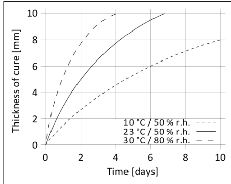
Diagram 1: Curing speed Sikaflex®-255 FC
