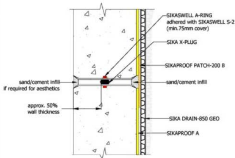
SIKAPROOF A (With Sleeve)
