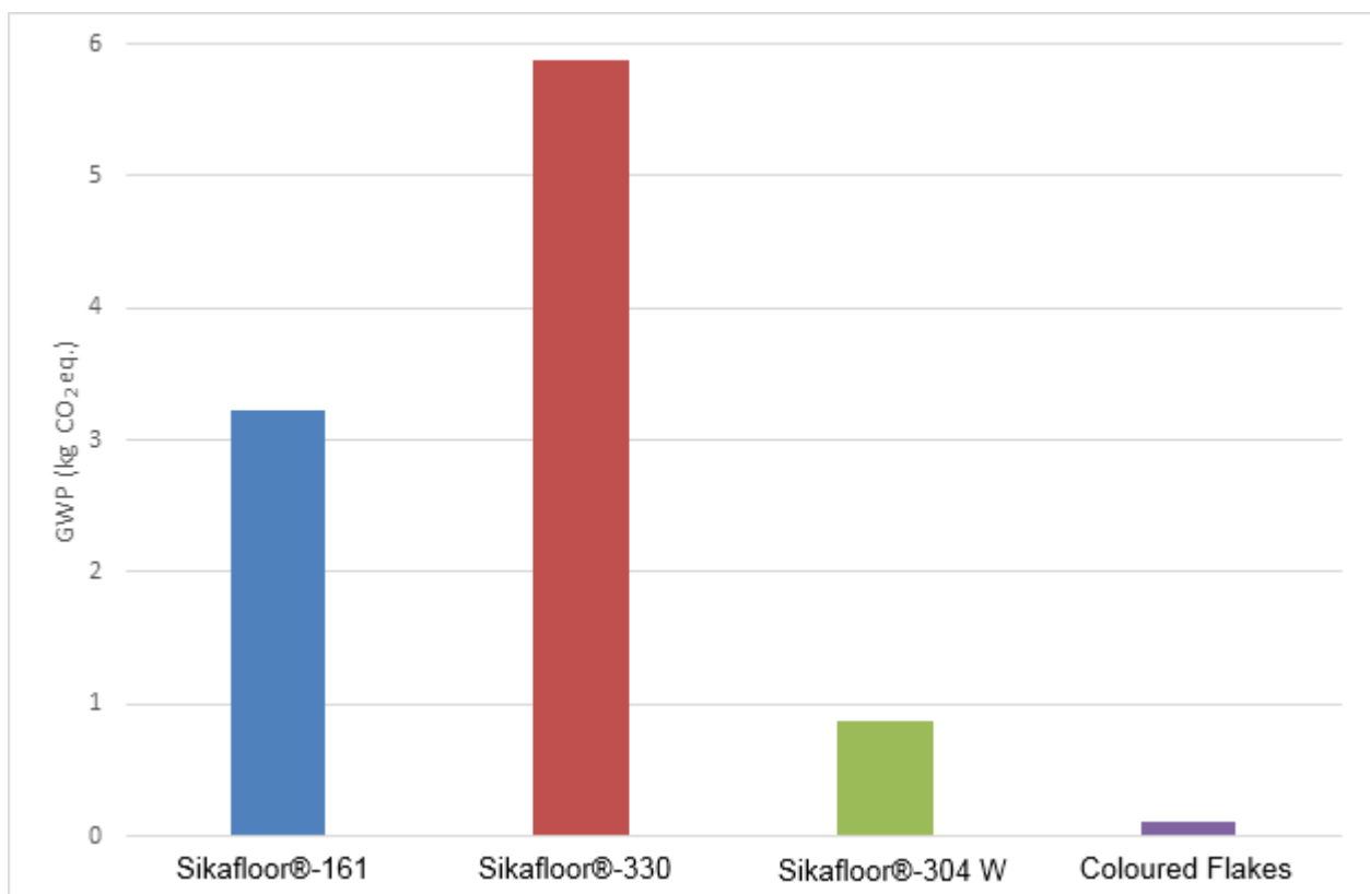
Figure 1: Sources of kg CO 2 equivalent impacts reported in the GWP for the product stage (A1 to A3) of Sika ComfortFloor® PS-24
