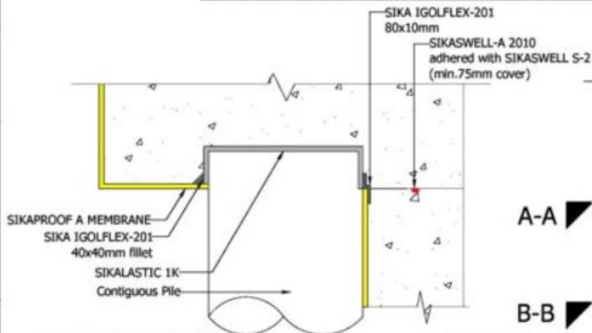
A-A SECTION THROUGH PILE
