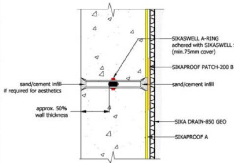
SIKAPROOF A (With Sleeve)
