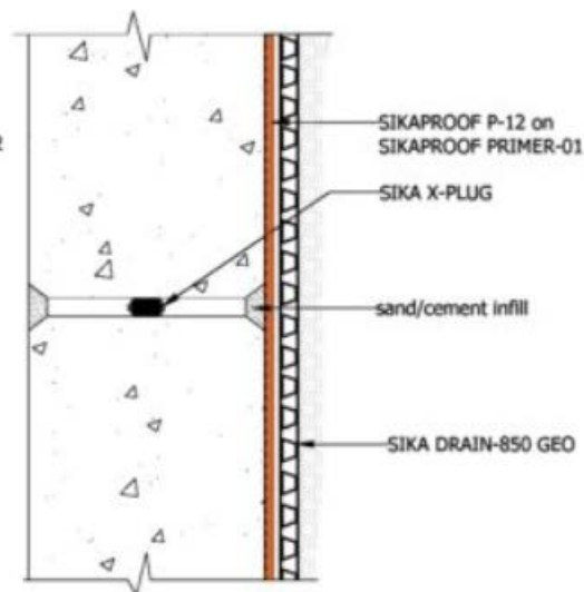
SIKAPROOF P-12 (Without Sleeve)
