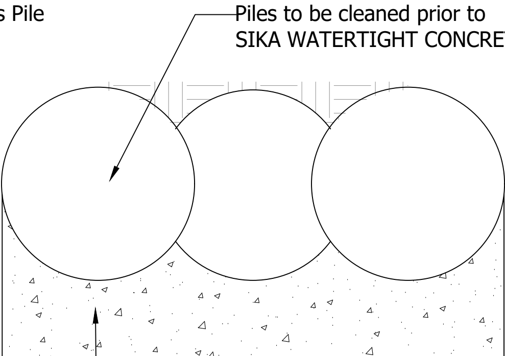
SIKA WATERTIGHT CONCRETE (min.200mm thickness)
