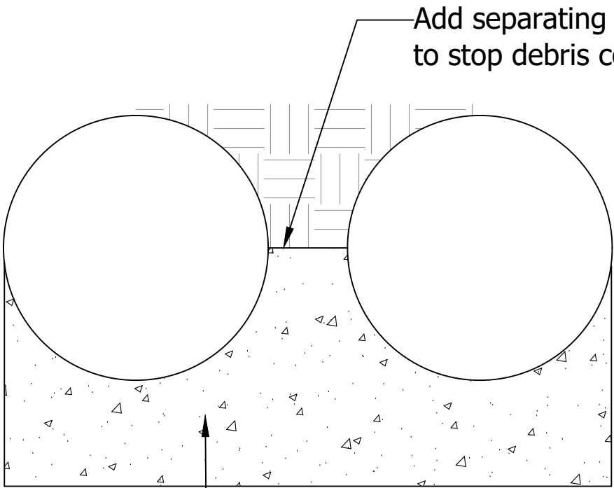
SIKA WATERTIGHT CONCRETE (min.200mm thickness)
