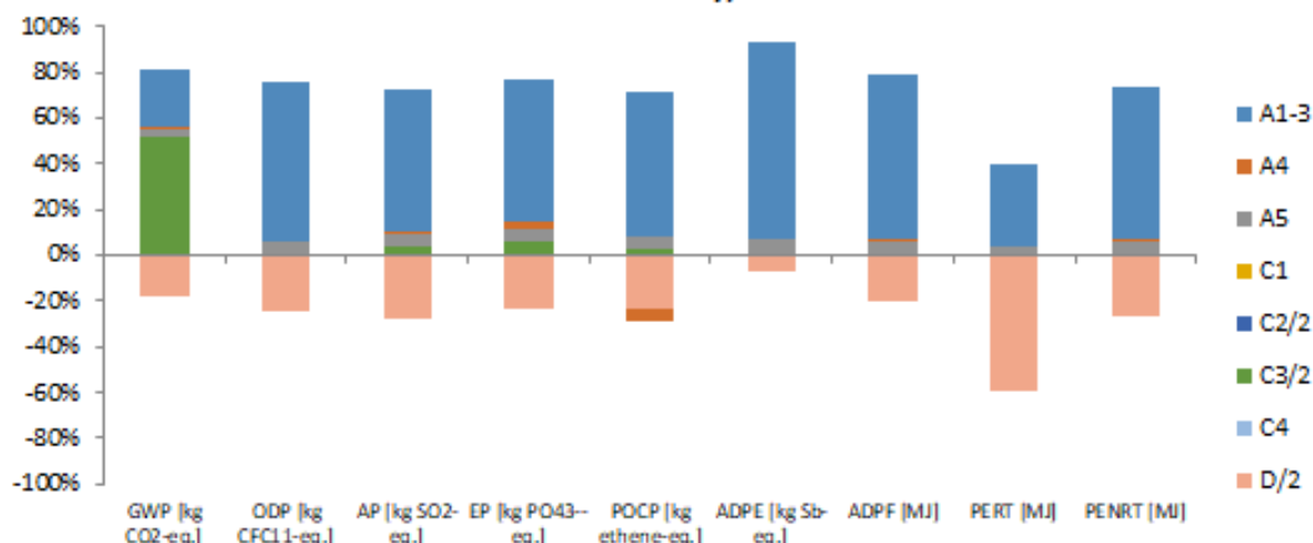
Relative contributions of the modules to environmental impacts and primary energy use of 1 m 2 Sarnafil TG 66-20 (100% thermal energy recovery)
