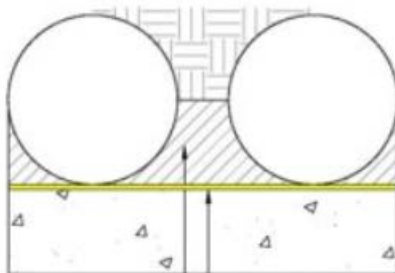
SIKAPROOF A back blinding/facing
