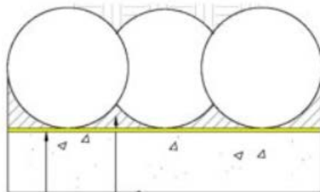
sacrificial formwork/facing to pile SIKAPROOF A
