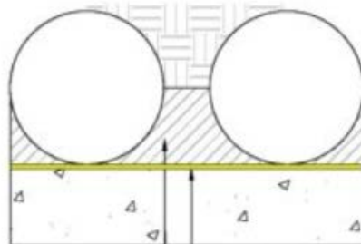
SIKAPROOF A back blinding/facing
