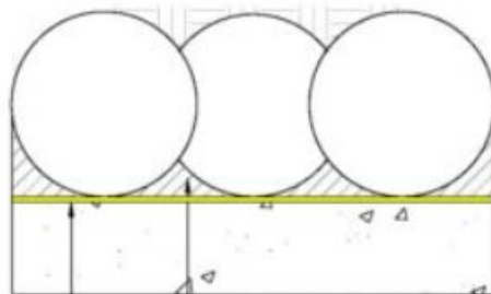
SIKAPROOF A sacrificial formwork/facing to pile
