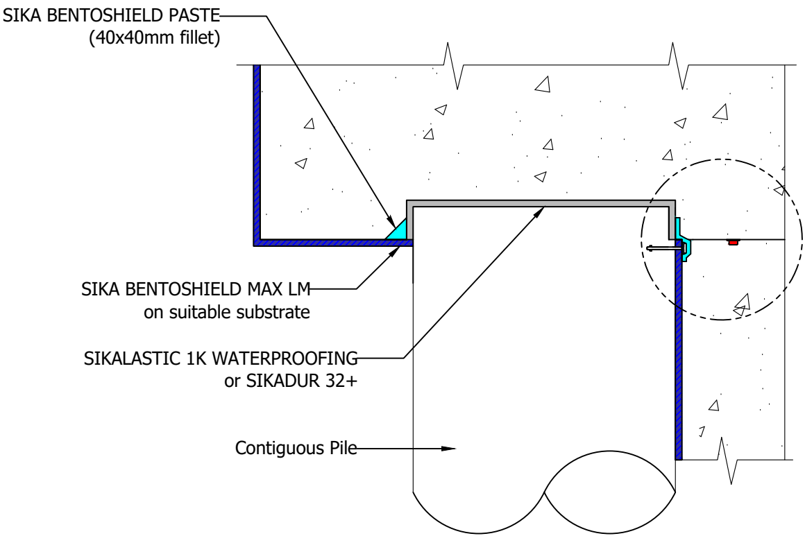
A-A SECTION THROUGH PILE
