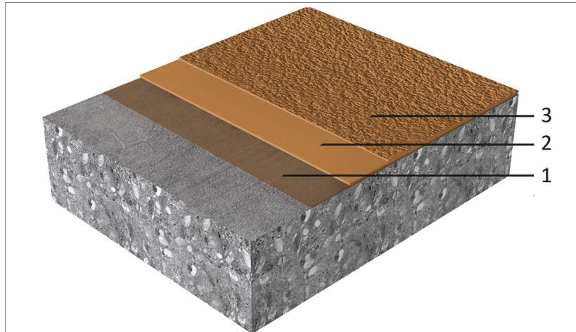
Sikafloor® Pronto RB-27 system (~ 3–5 mm)
